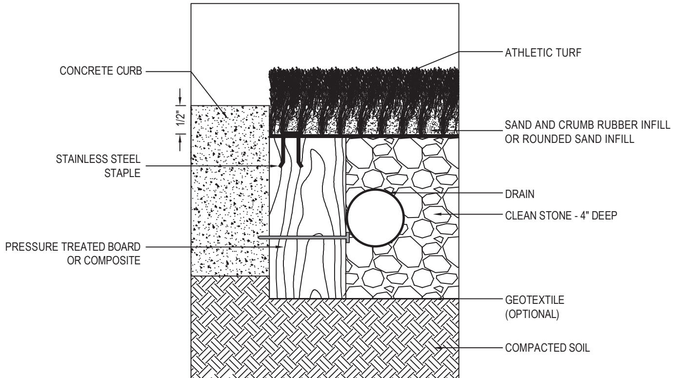
INSTALLATION WITH CURB
