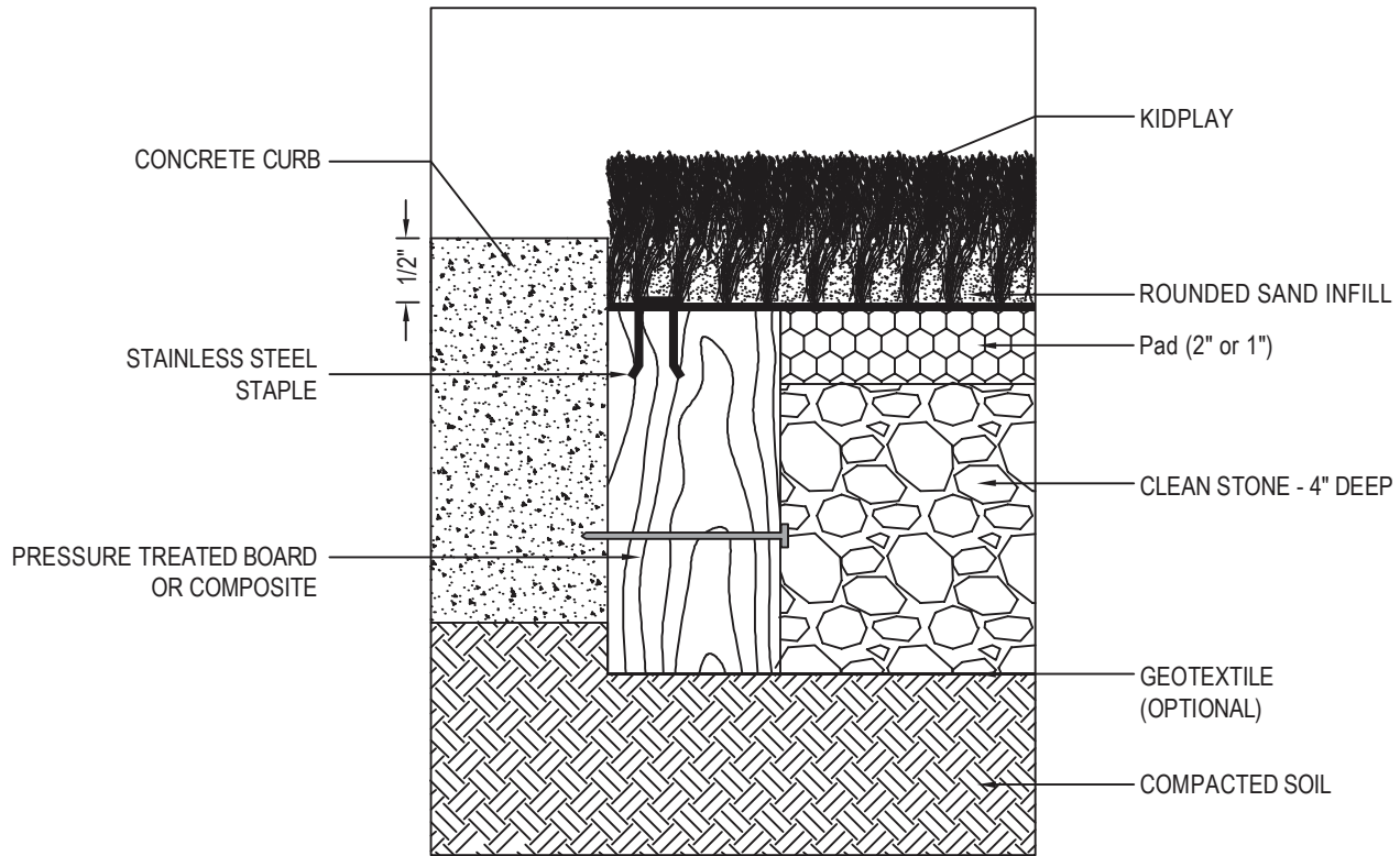
INSTALLATION WITH CURB
